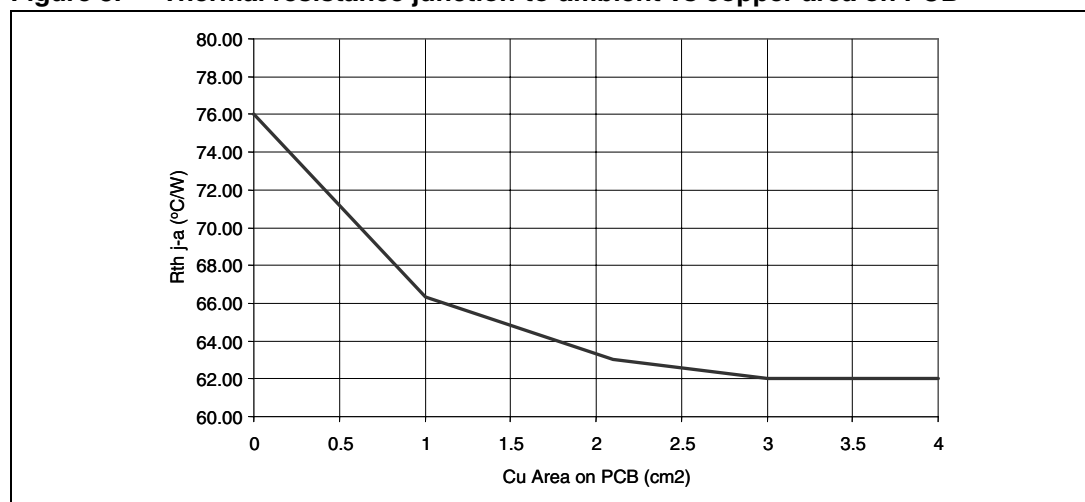
Figure 3. Thermal resistance junction-to-ambient vs copper area on PCB
